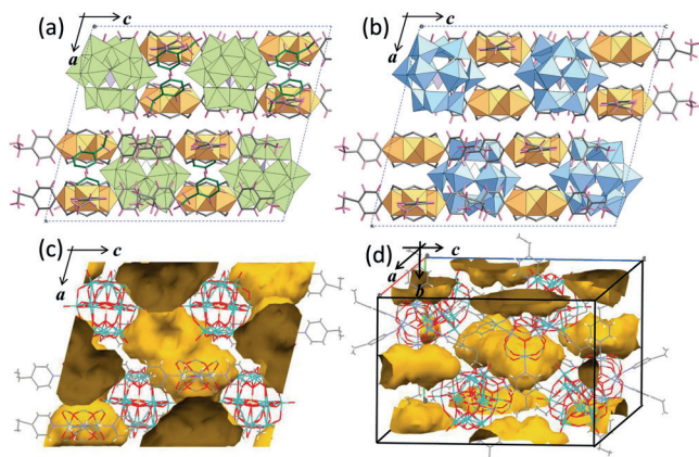
Figure 1. a) Crystal structure of I-as . b) A model structure of I-red constructed by removing one of the three \text{etpy} ligands in the macrocation and the \text{etpyH}^+ ion from (a). c) and d) Void analysis of I-red with a probe radius of 1.2 Å viewed from different directions. Green and blue polyhedra show the [\text{MoO}_6] units of fully oxidized and reduced POM, respectively. Orange and purple polyhedra show the [\text{CrO}_5\text{N}] units of macrocation and [\text{SiO}_4] units of POM, respectively. Aromatic rings of \text{etpy} ligands of the macrocation and \text{etpyH}^+ are drawn in gray and green, respectively. In (c) and (d), void spaces are shown in brown. Each void has a size of about 6.5 by 12.5 Å.
